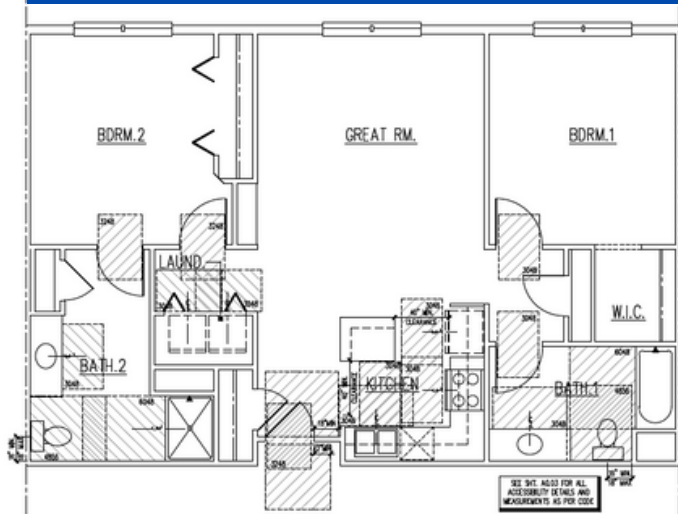
UNIT PLAN 2BR-D
